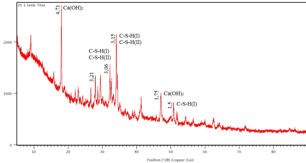
Data of X-ray phase analysis of cement stone without additives.
