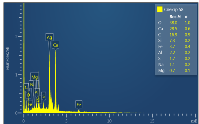
Microstructure and composition of cement stone MS
