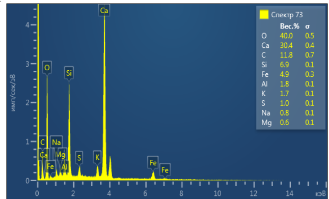
Microstructure and composition of cement stone MS
