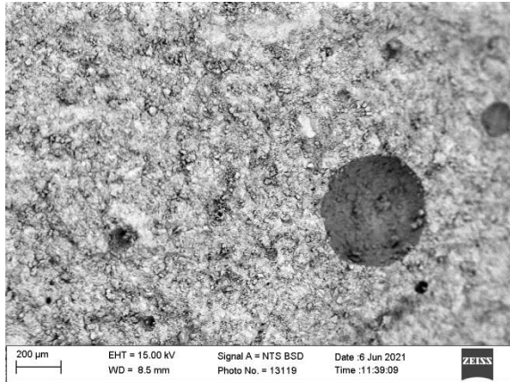
Microstructure and composition of cement stone without additives.
