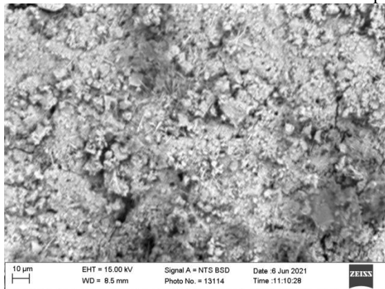
Microstructure and composition of cement stone MS
