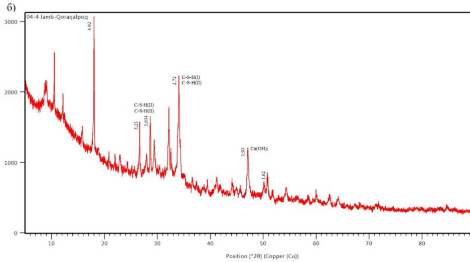
Data of X-ray phase analysis of cement stone without additives.
