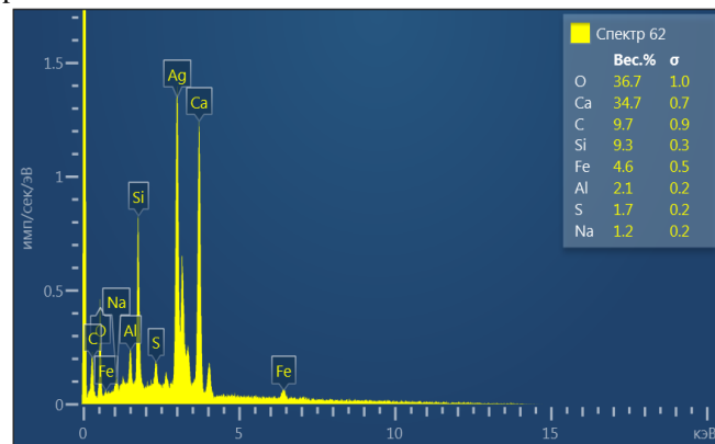
Microstructure and composition of cement stone SP+MS+MH
