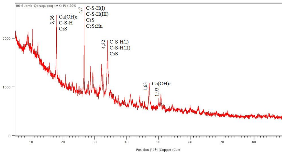
Data of X-ray phase analysis of cement stone SP+ MS + MH
