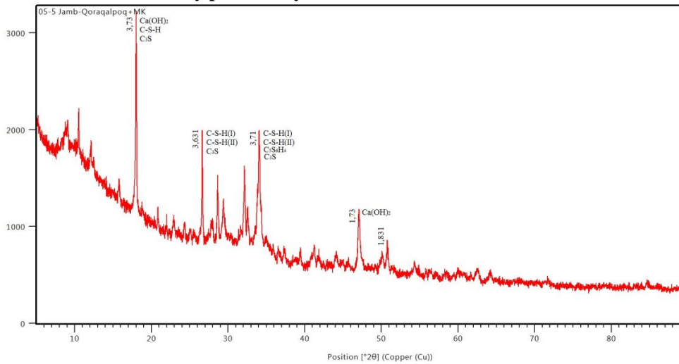
Data of X-ray phase analysis of cement stone +MS
