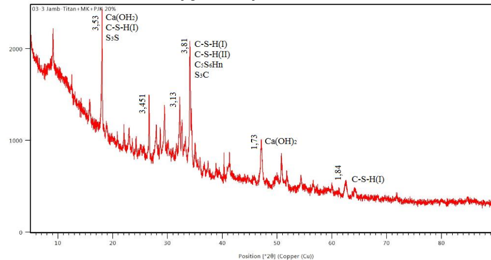
Data of X-ray phase analysis of cement stone SP + MS + MH
