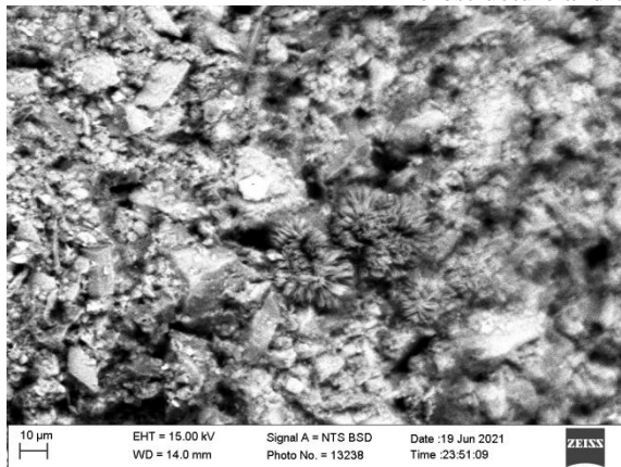
Microstructure and composition of cement stone SP+MS+MH
