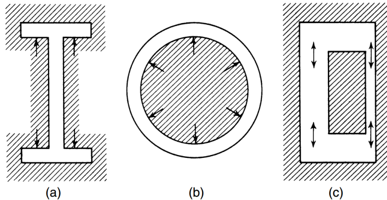
Figure 5. Typical design features giving rise to contraction stresses. (a) Mould restraint, (b) core restraint, (c) differential contraction of casting members
