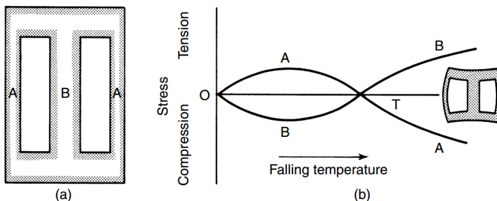
Figure 6. Development of stresses through differential contraction. (a) Stress grid casting (b) schematic plot of stresses in thick and thin members, illustrating change in sign during cooling
