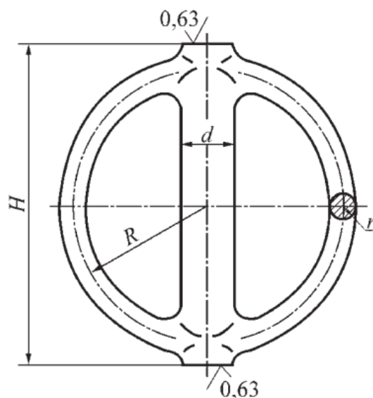
Figure 7. Sample lattice for determining residual stresses.
