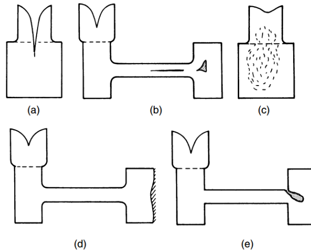
Figure 1. Forms of shrinkage defect. (a) Primary pipe, (b) secondary cavities, (c) discrete porosity, (d) sink, (e) puncture
