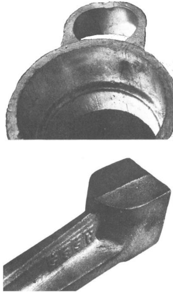
Figure 4. Two examples of shrinkage puncture or 'draw'
