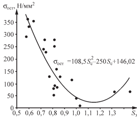
Fig. 8. The influence of the degree of eutecticity of white chromium cast irons on the level of residual stresses
