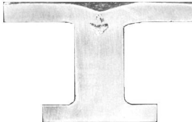
Figure 3. Sectioned casting exhibiting internal shrinkage cavity and sink
