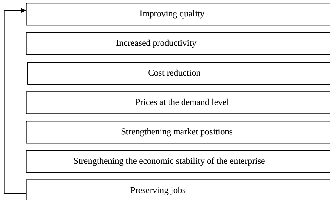
Figure 6. "Chain reaction" by E. Deming
